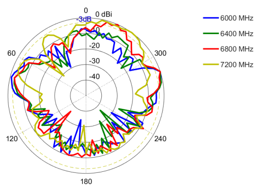
Elevation 1: 6000 – 7200 MHz
