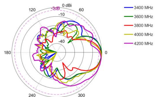
Elevation: 3400 – 4200 MHz
