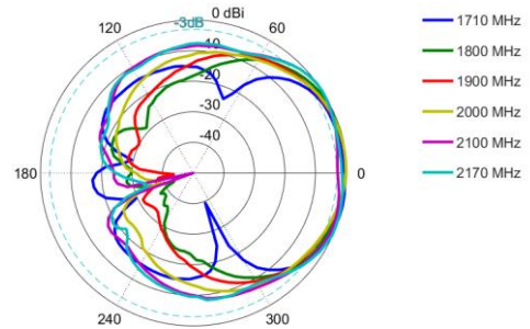
Elevation: 1710 – 2170 MHz
