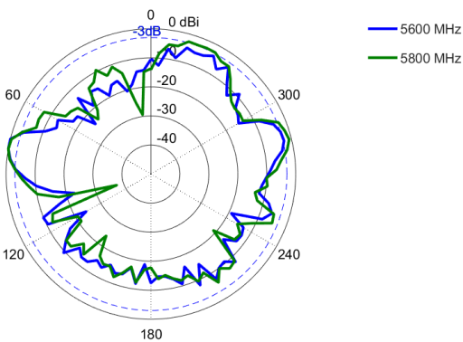
Elevation 2: 5600 – 5800 MHz
