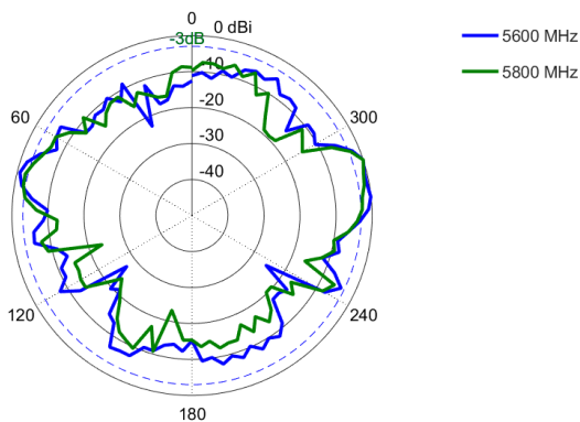
Elevation 1: 5600 – 5800 MHz
