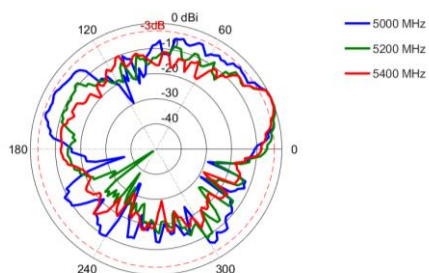
Elevation: 5000 – 5400 MHz
