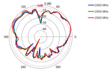
Elevation: 2400 – 2500 MHz
