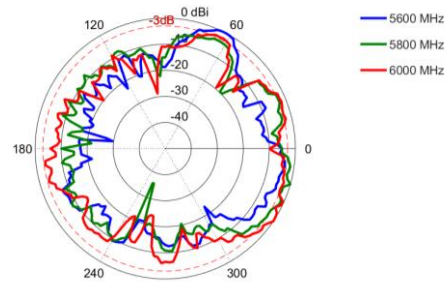
Elevation: 5600 – 6000 MHz
