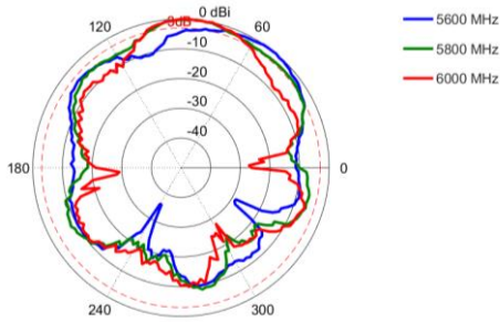
Azimuth: 5600 – 6000 MHz
