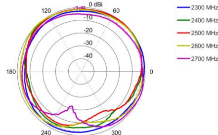
Azimuth: 2300 – 2700 MHz
