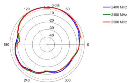
Elevation 2: 2400 – 2500 MHz
