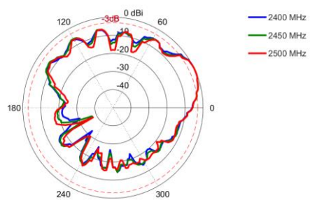
Elevation 2: 2400 – 2500 MHz
