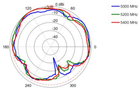
Azimuth: 5000 – 5400 MHz
