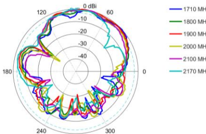
Elevation 2: 1710 – 2170 MHz
