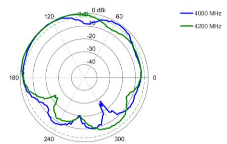
Elevation 2: 4000 – 4200 MHz
